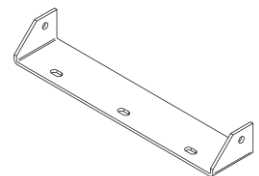
(1) B2539 BOOT PLATE
