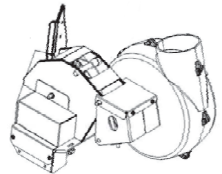
(1) A0739 PTO ASSEMBLY
