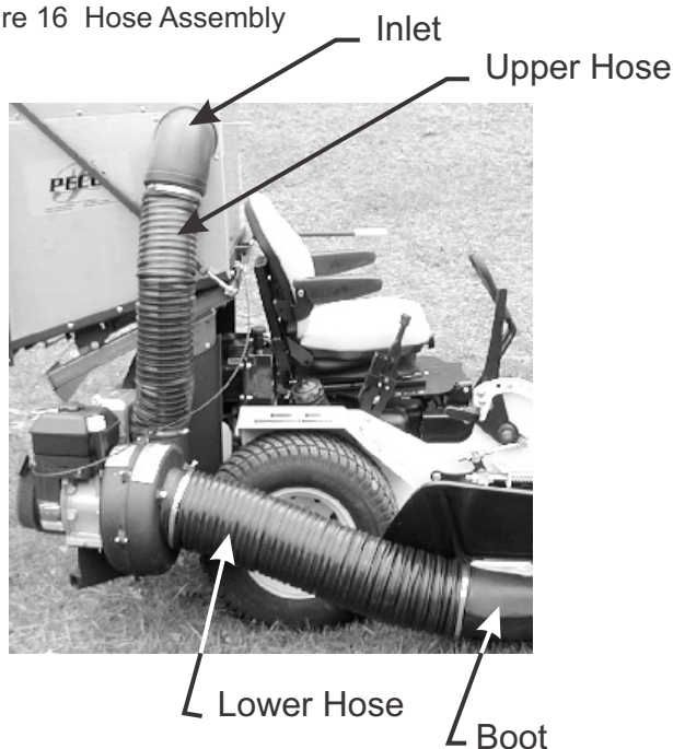
Figure 16 Hose Assembly
