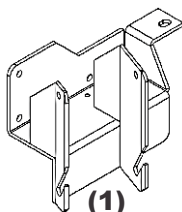
(1) A0846 PTO MOUNT PLATE ASSY.
