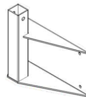
(1) A0617 LWR. MNT. ASSEMBLY
