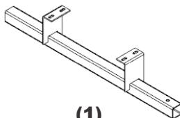
(1) A0110 OUTER MOTOR MOUNT TUBE
