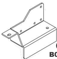
(1) B0396 RT. LWR. MOUNT PL.
