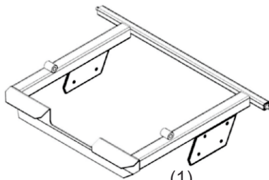
(1) A0452 TOP FRAME ASSY.
