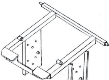
(1) A0319 MAIN FRAME ASSY.
