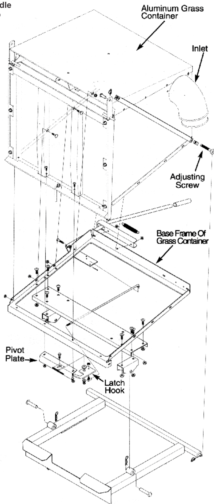
Figure 6 Aluminum Grass Container Assy.
