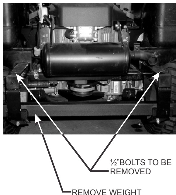
Figure 1 Bolt Removal
