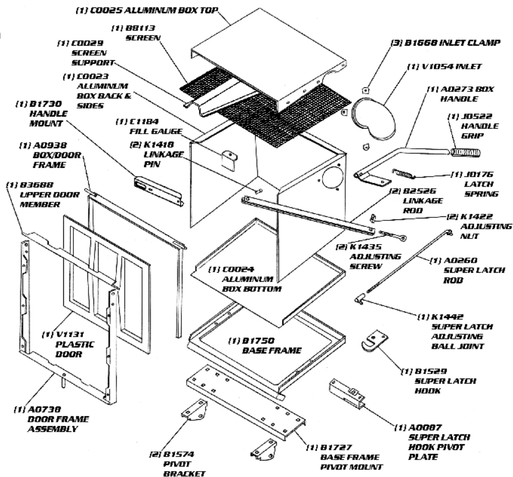
Figure 7 Aluminum Grass Container Exploded View
