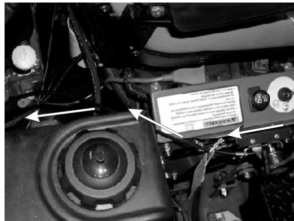
Figure 17 Throttle Cable Routing
