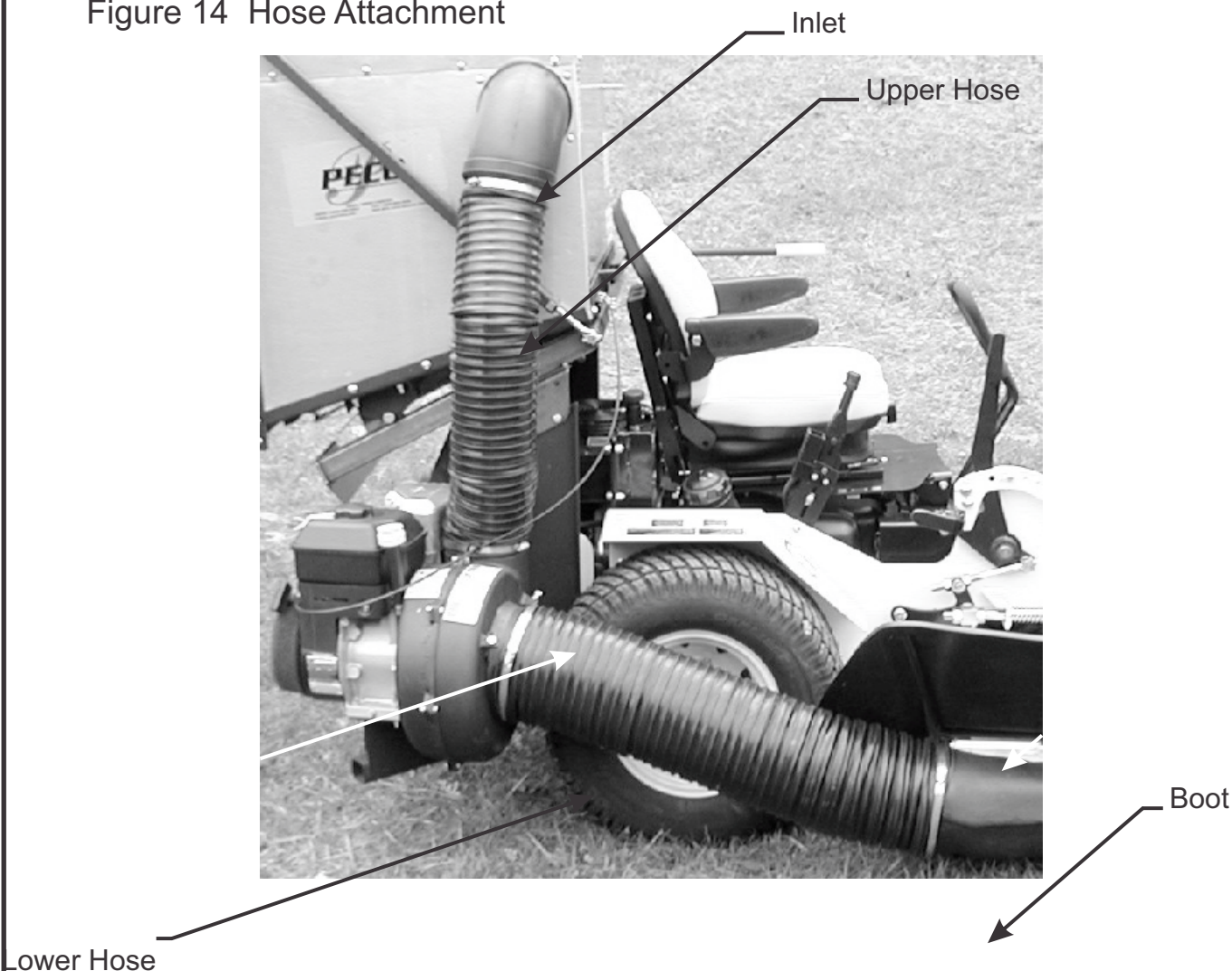
Figure 14 Hose Attachment
