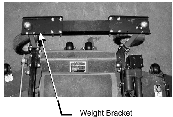
Figure 18a Bobcat Weight Kit Bolt Pattern
