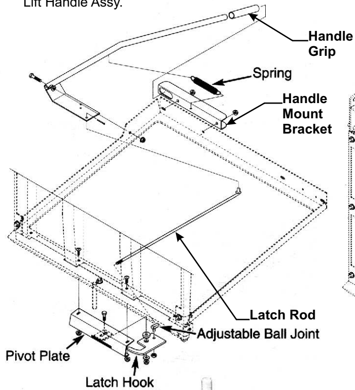
Figure 7 Aluminum Grass Container With Handle Attached
