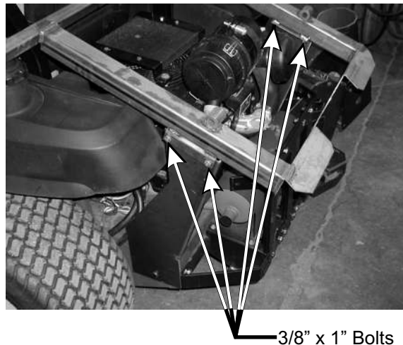
Figure 5 Top Main Frame Assy.
