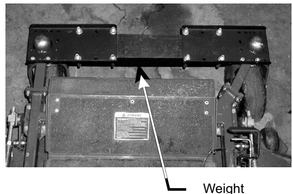
Figure 18b Bunton Weight Kit Bolt Pattern
