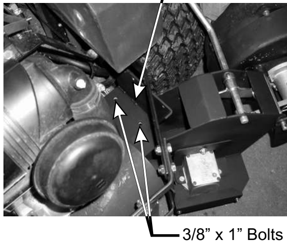
Figure 4-1 PTO Arm Assy. 3/8" x 1" Bolt
