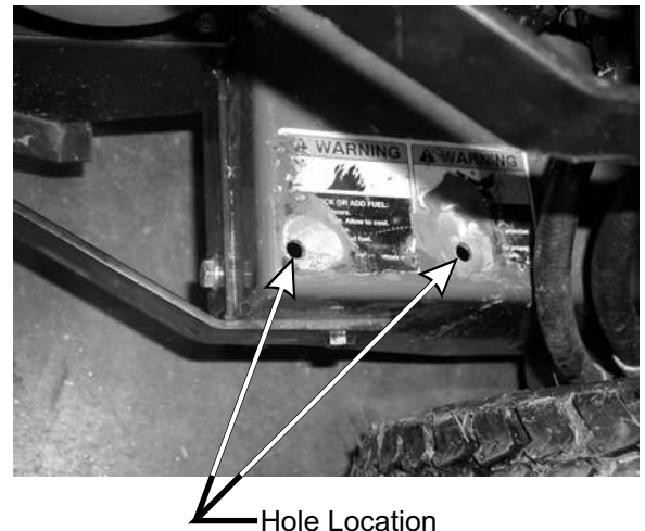
Figure 3 Heat Guard
