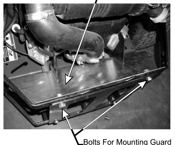
Figure 3 Heat Guard
