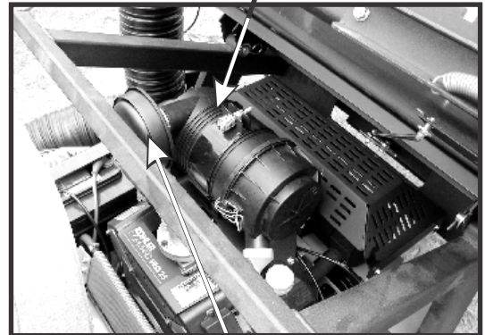
Donaldson Air Cleaner Rotated To Forward Position
