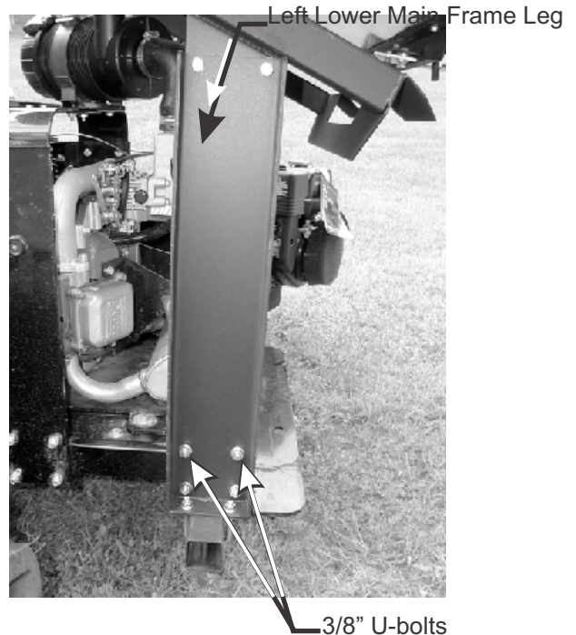
Figure 1 Left Lower Main Frame Leg.
