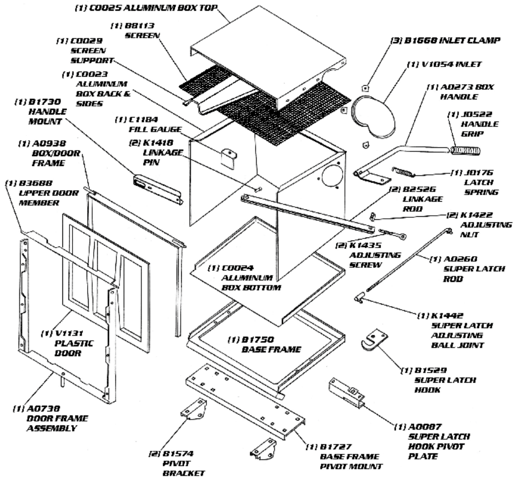
Figure 9 Aluminum Grass Container Exploded View
