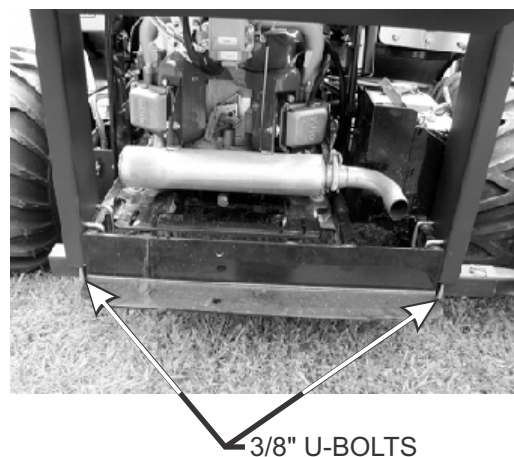
Figure 3 Outer Motor Mount Tube Attachment
