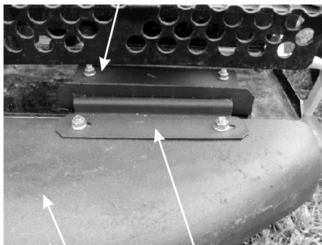
Boot Plate
