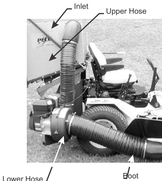
Figure 16 Hose Assembly
