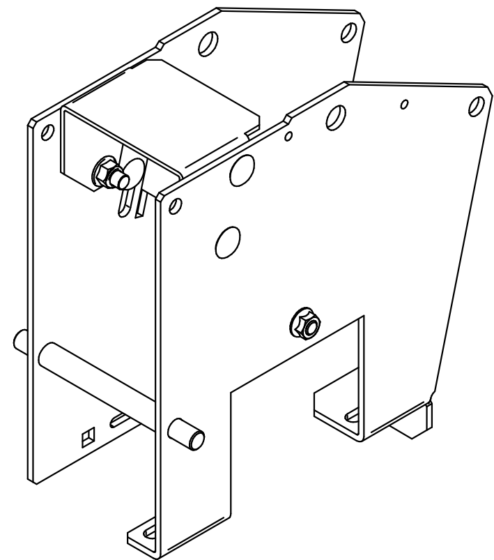
Iso View
