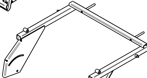
(1) A0579 BOX SUPPORT FRAME ASSY
