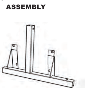
(1) A0605 OUTER ENGINE MNT. TUBE ASSY.
