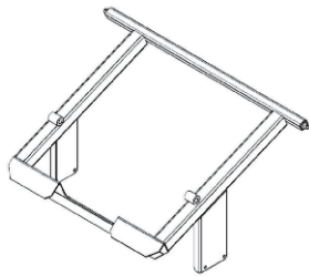
(1) A0680 MAIN FRAME ASSY.
