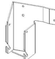
(1) B0272 PTO ASSY. MOUNT PLATE
